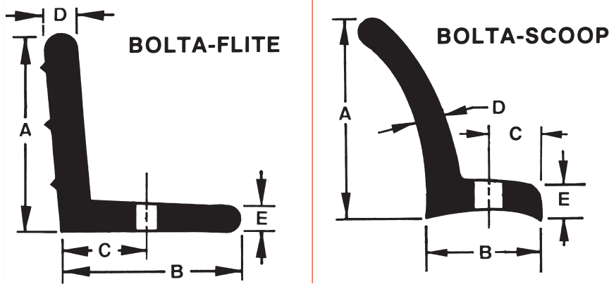
FIGURE 4: CLEAT CROSS-SECTIONS
