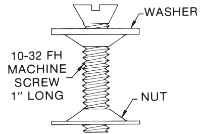
Fig. 5. Bolta-Flite and ① ③ Bolta-Scoop Hardware
